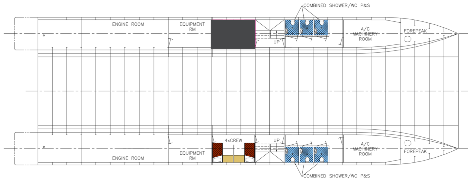
MAIN DECK
