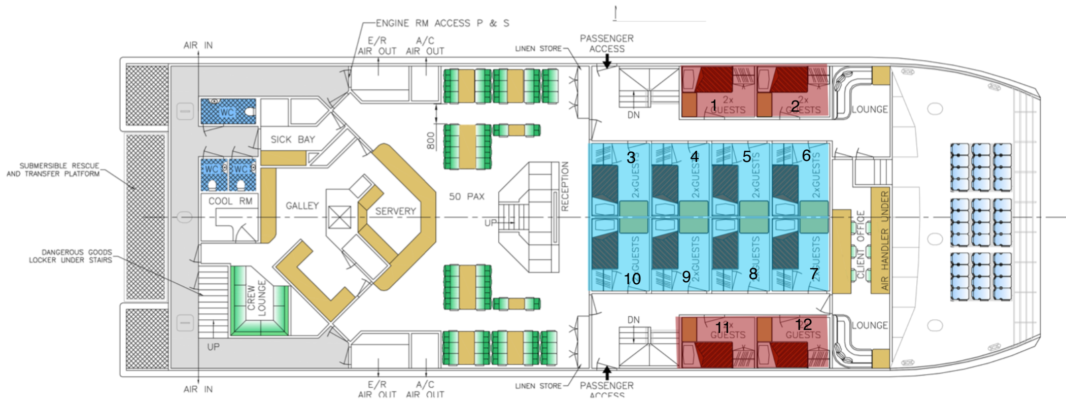
MAIN DECK
